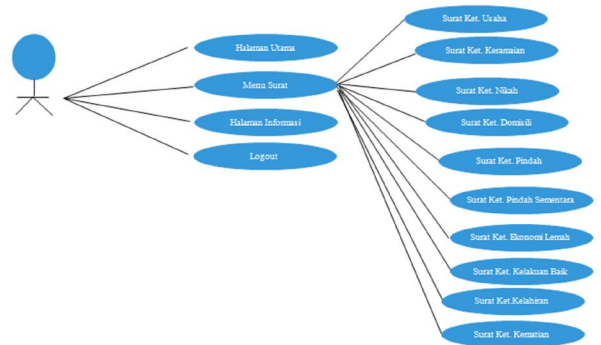
Gambar 3. Usecase Diagram User
