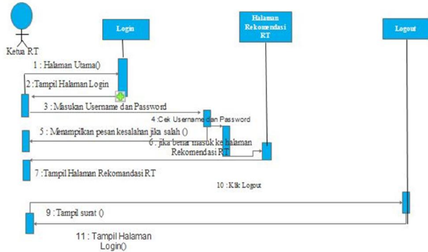
Gambar 6. Sequence Diagram Dusun
