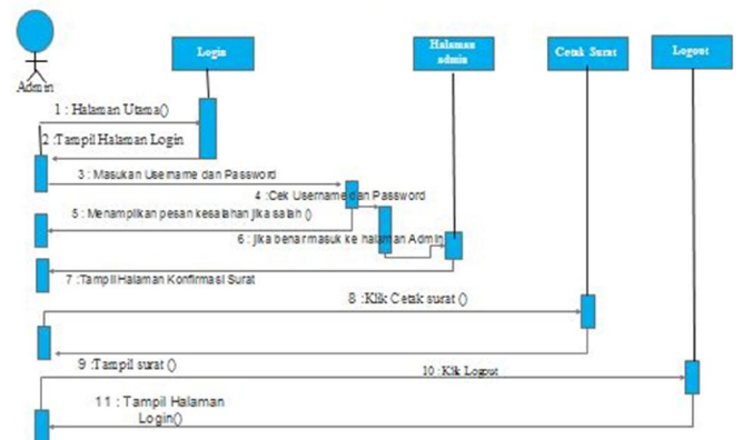
Gambar 5. Sequence Diagram Admin
